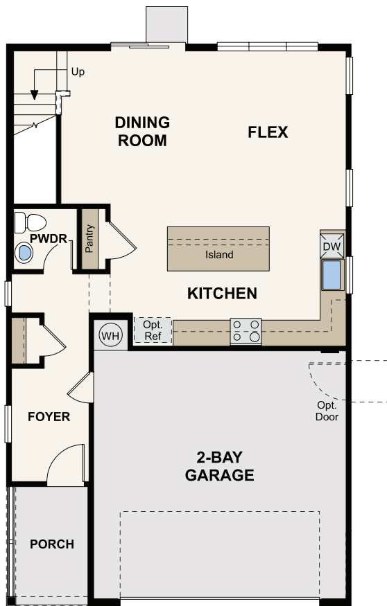
MAIN LEVEL
